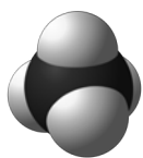
\text{CH}_4 methane
