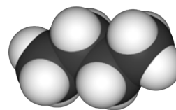
\text{C}_4\text{H}_{10} butane
